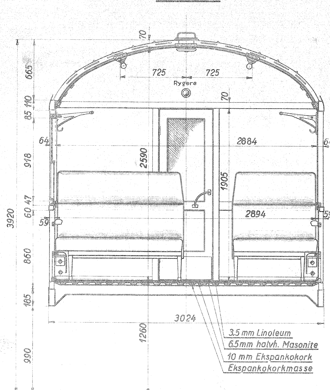
Snit: C-C
