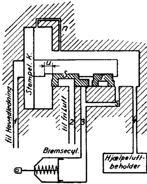
b. Bremsestilling.
