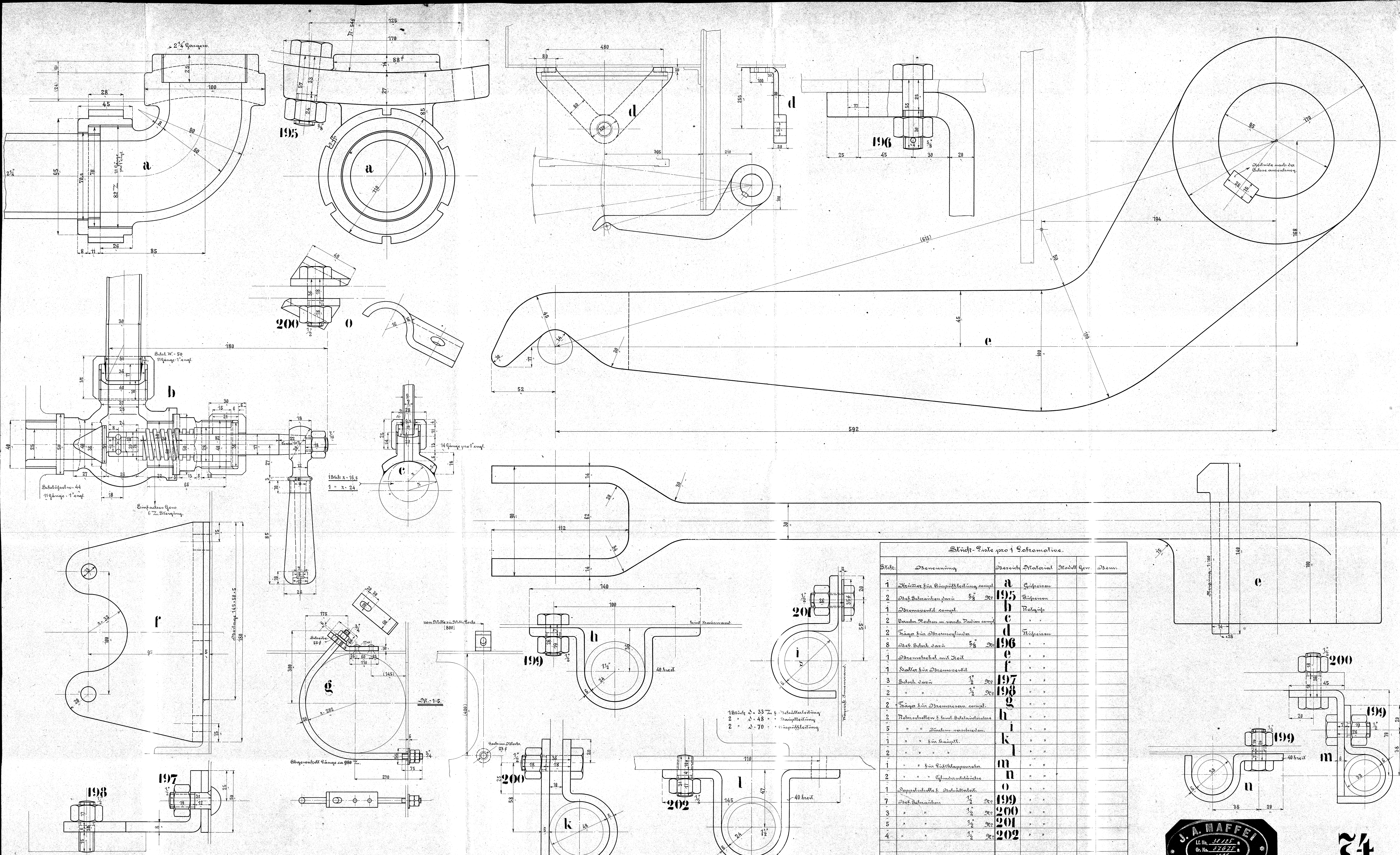
Safetybrake-Details.
